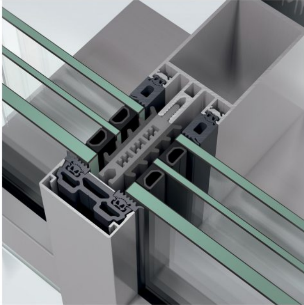
AluClear Facade System FWS 50.SI Green
