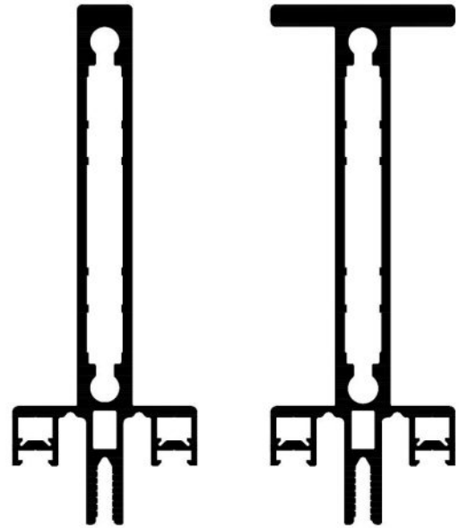
Horizontal section detail of AluClear Facade System FWS 50 S
