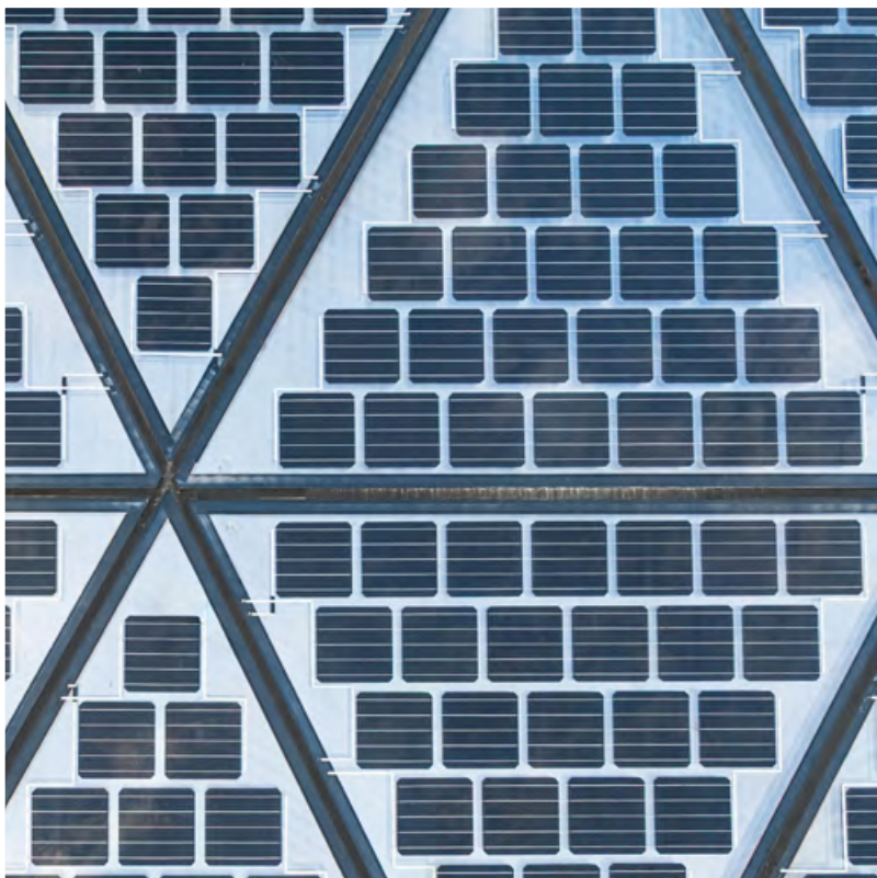
AluClear products: BIPV Skylight Opaque glass-glass modules
