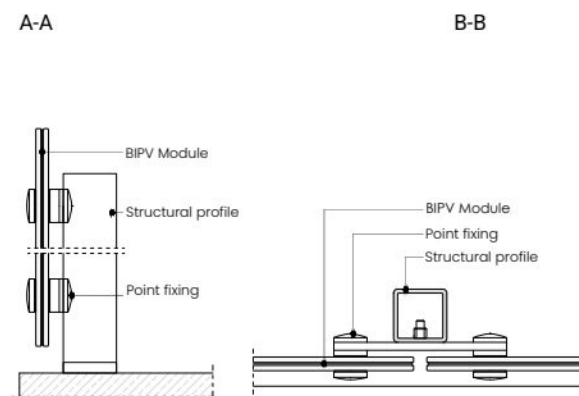
POINT-MOUNTED BALUSTRADE
