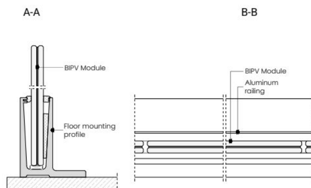
SELF-SUPPORTING BALUSTRADE
