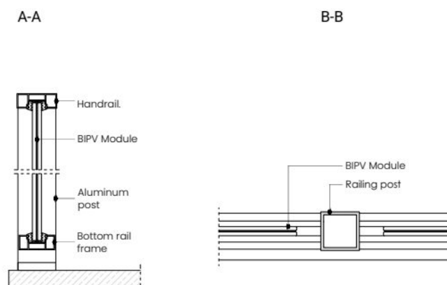
BALUSTRADE WITH HANDRAIL
