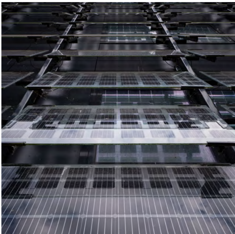
AluClear products: BIPV roof glazing transparent glass-glass modules
